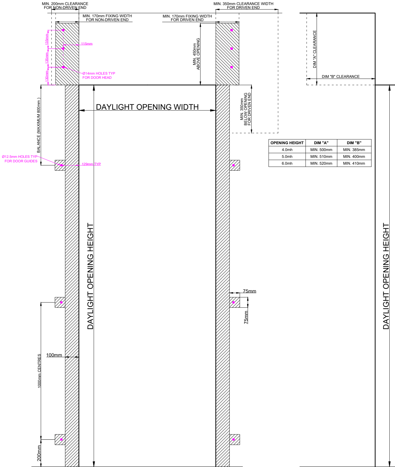
FRONT VIEW (FROM INSIDE BUILDING)
