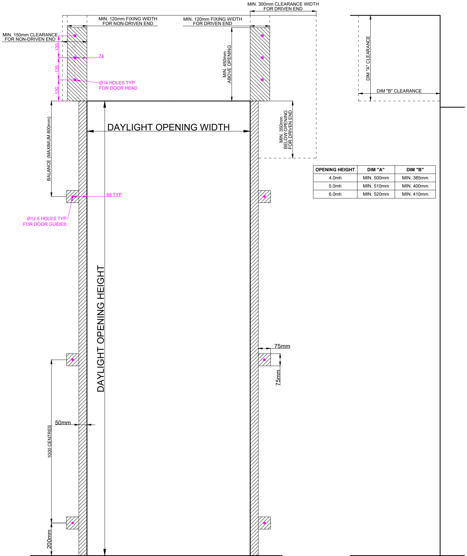
FRONT VIEW (FROM INSIDE BUILDING)
