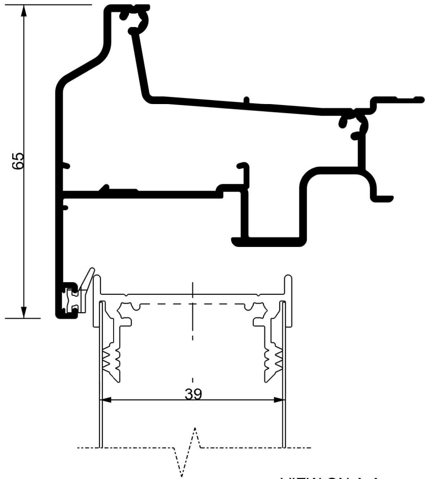
VIEW ON A-A
