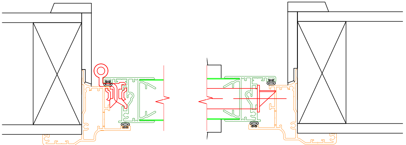
SECTION B-B
