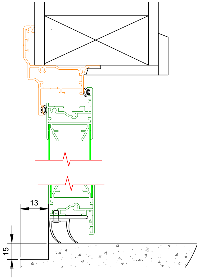
VIEW ON A-A (SILL OPTION 1)
